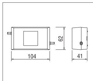
MAW-B Auxiliary light control relay
